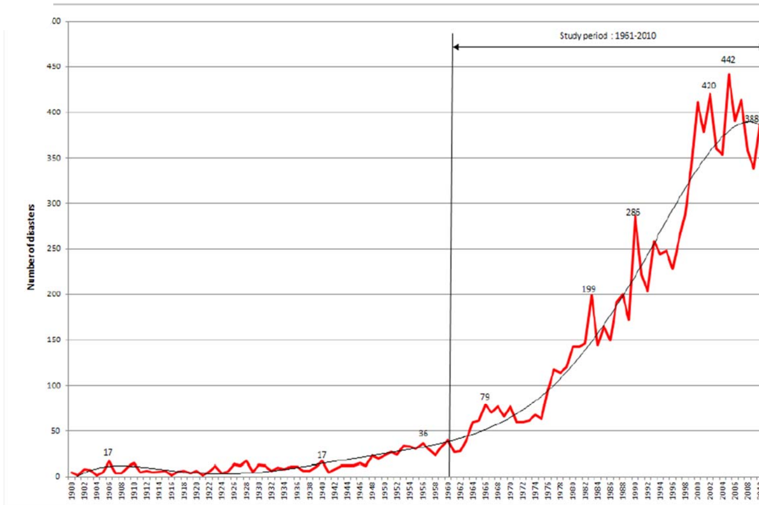
Occurrence of natural disasters as reported in EMDAT: 1900 – 2010
